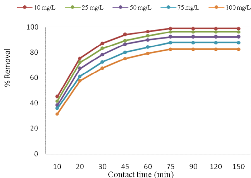
Fig 2. Effect of contact time and concentration on AG25 removal (pH =7, Adsorbent dosage 3 g/L and temperature = 28± 2°C)
