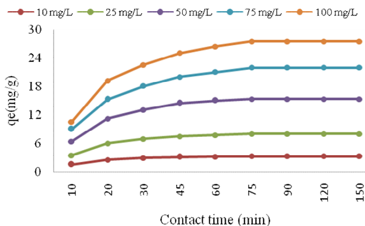
Fig 3. Effect of contact time on adsorption capacity (pH =7, Adsorbent dosage 3 g/L and temperature = 28 \pm 2 °C)
