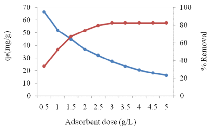
Fig 4: Effect of adsorbent dosage on AG25 adsorption. ( C_0 = 100 mg/L, time = 75 min, pH = 7, temp = 28 \pm 2 °C)
